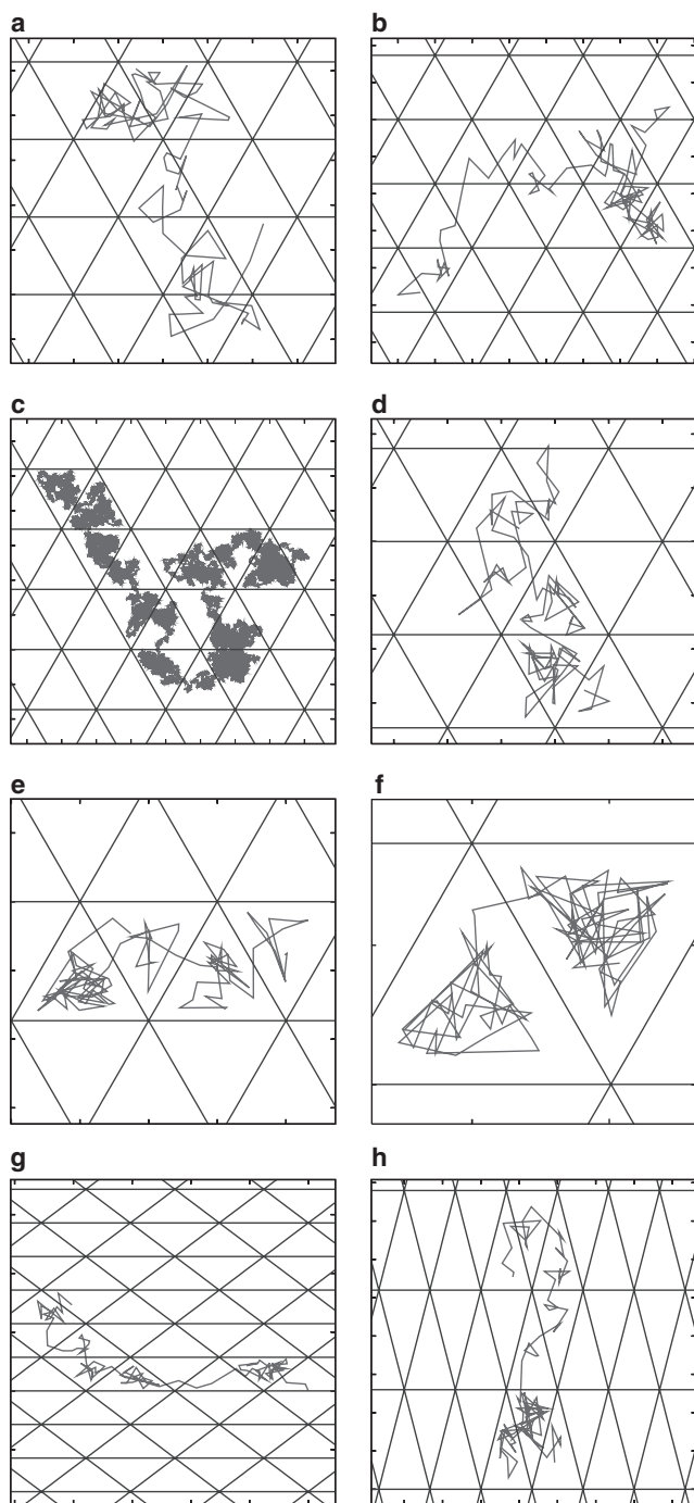
FIGURE 3 Simulation snapshots of a particle diffusing within the lipid bilayer under influence of the potential landscape that is defined by the cytoskeletal pressure. Cytoskeletal bonds have an unstretched bond length d = 100 nm and are sketched using straight lines; for better visibility the coarse-grained path of the diffusing particle connects the particle positions only every 1000 simulation steps (except subfigure (c)). The length of the overall path is 100,000 simulation steps each. All plots show a square region of the cell membrane, the tick distance is 50 nm. Snapshots are plotted for the unstretched cytoskeleton and several effective interaction volumes of the diffusing particle, v , as well as for two stretched cytoskeletons: (a) unstretched, v = 2000 nm 3 ; (b) unstretched, v = 6000 nm 3 ; (c) unstretched, v = 6000 nm 3 , position shown every simulation step; (d) unstretched, v = 10,000 nm 3 ; (e) unstretched, v = 20,000 nm 3 ; (f) un-
